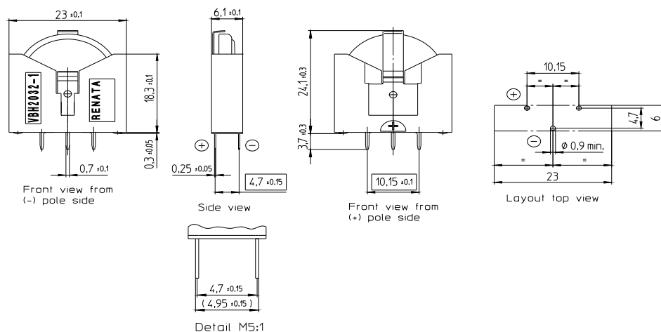
Dimensions (mm)
