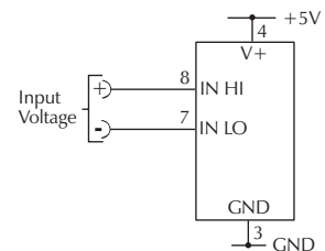
Check solder link 2 is SHORTED.
