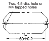
Mounting Holes
