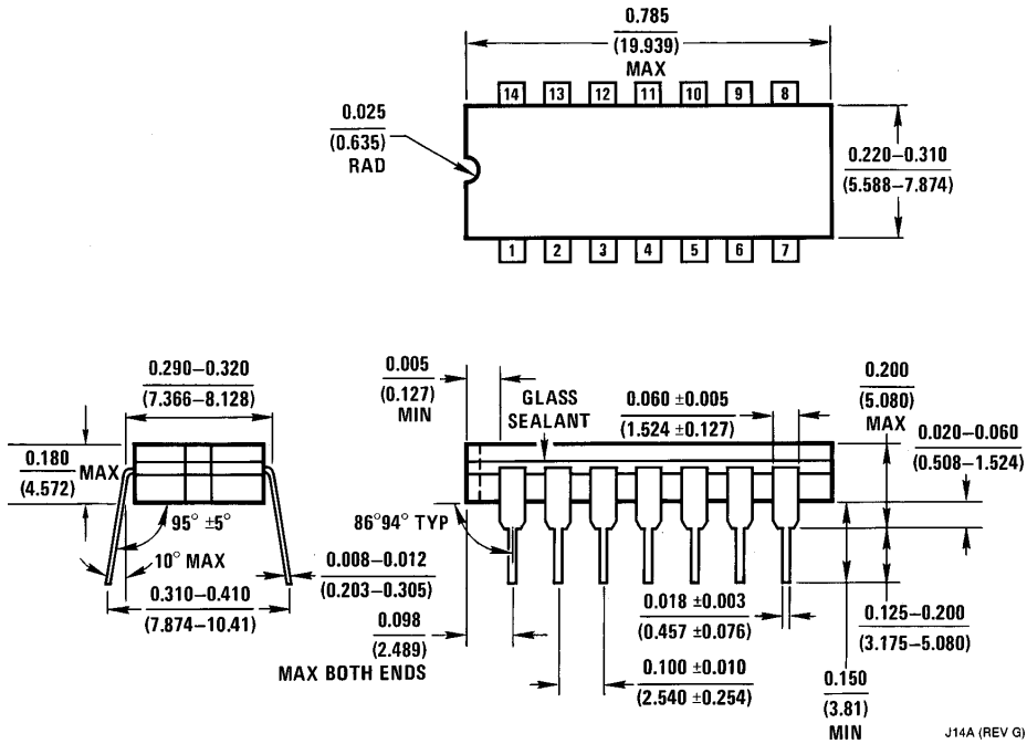
14-Pin Ceramic Dual-In-Line Package Order Number LMC6484AMJ/883 NS Package Number J14A
