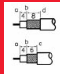
Adjusted blades strip to these specifications for RG58/RG59/RG62/RG6 and RG8/RG11/RG213
