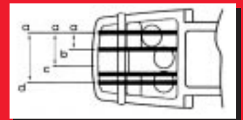
Detail of blades in stripping jaw showing three-level strip
