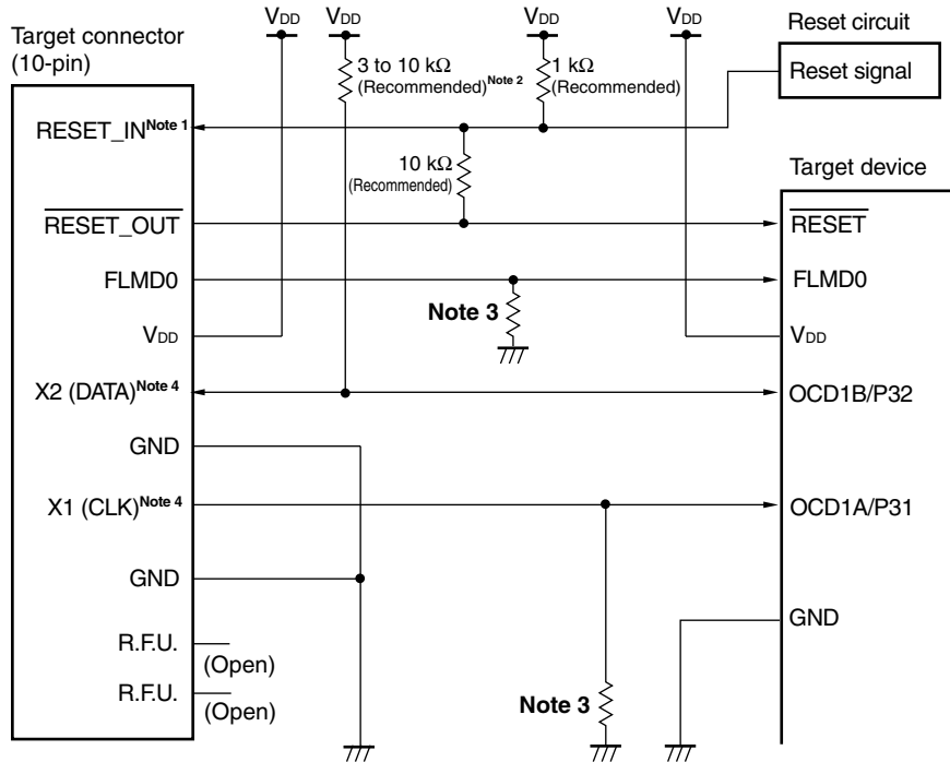
Figure 22-2. Connection Example of QB-78K0MINI or QB-MINI2 and μPD78F0503D (When OCD1A/P31 and OCD1B/P32 Are Used)
