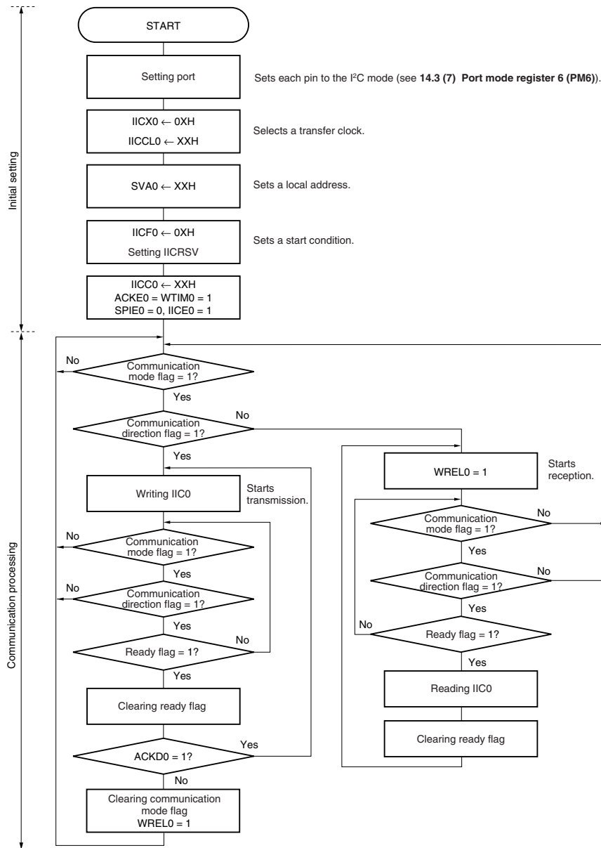
Figure 14-25. Slave Operation Flowchart (1)
