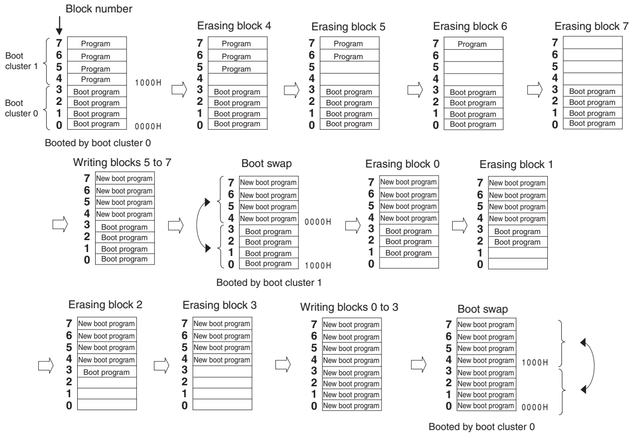
Figure 21-16. Example of Executing Boot Swapping
