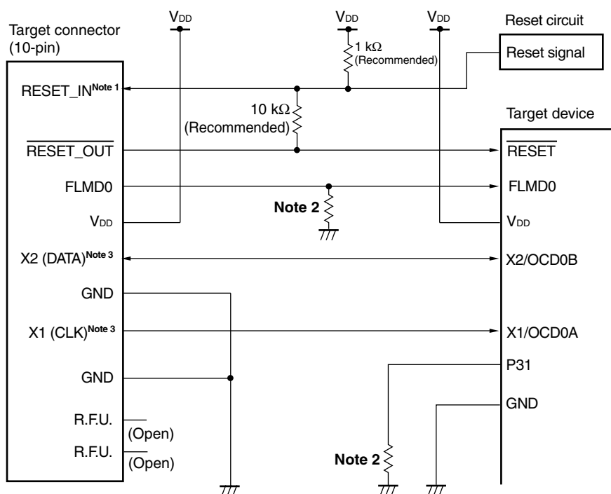
Figure 22-1. Connection Example of QB-78K0MINI or QB-MINI2 and \mu PD78F0503D (When OCD0A/X1 and OCD0B/X2 Are Used)
