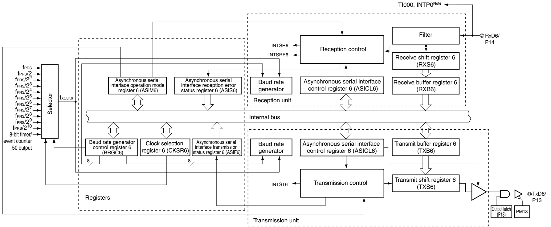
<R>Figure 12-4. Block Diagram of Serial Interface UART6
