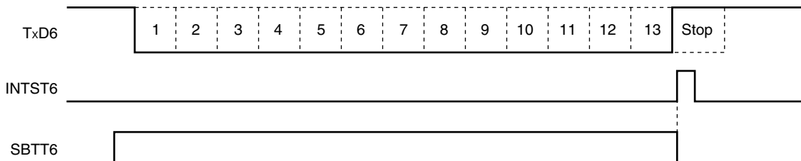
Figure 12-22. SBF Transmission
