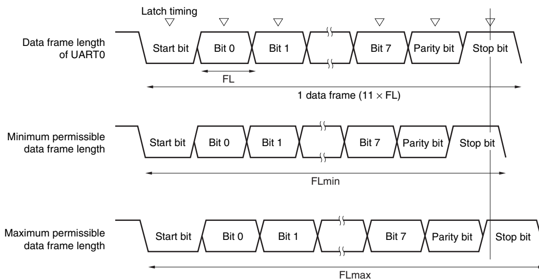
Figure 11-12. Permissible Baud Rate Range During Reception
