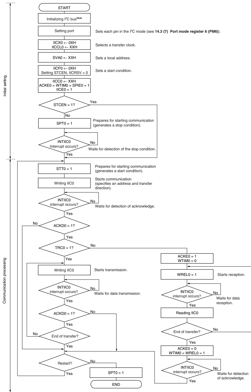
Figure 14-23. Master Operation in Single-Master System
