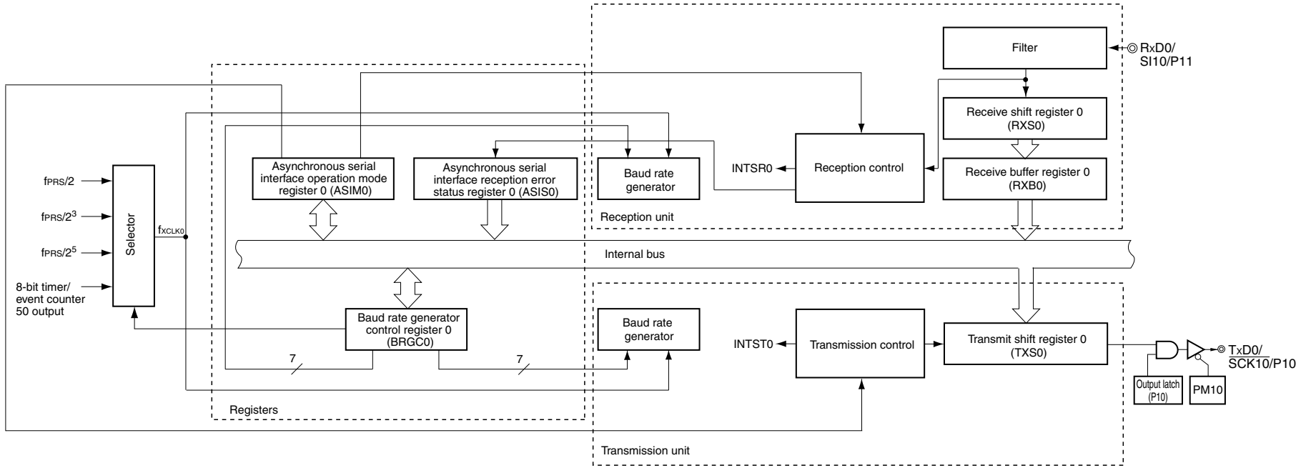
<R> Figure 11-1. Block Diagram of Serial Interface UART0
