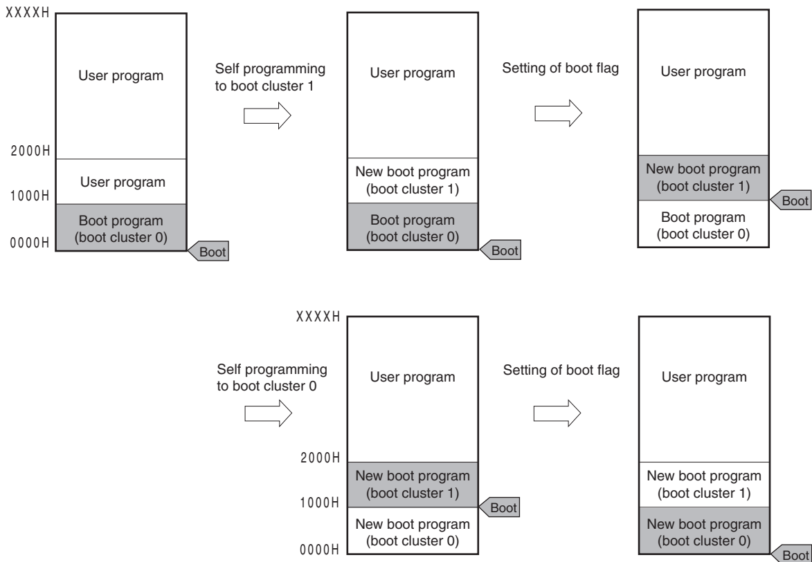
<R> Figure 21-15. Boot Swap Function
