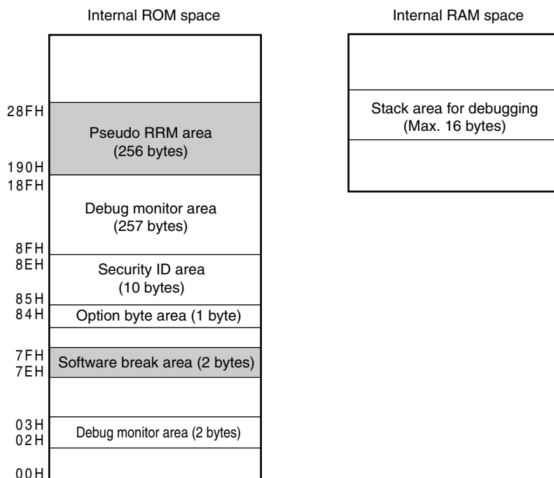
Figure 22-4. Reserved Area Used by QB-78K0MINI and QB-MINI2
