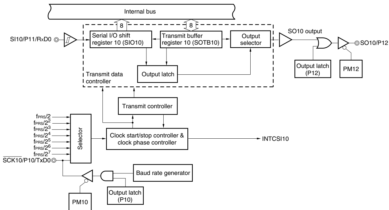
Figure 13-1. Block Diagram of Serial Interface CSI10
