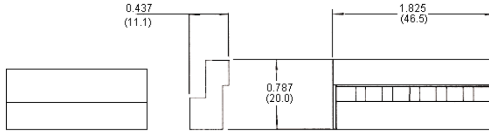
Pattern A for Use on Bobbin Sizes 29 and 196
