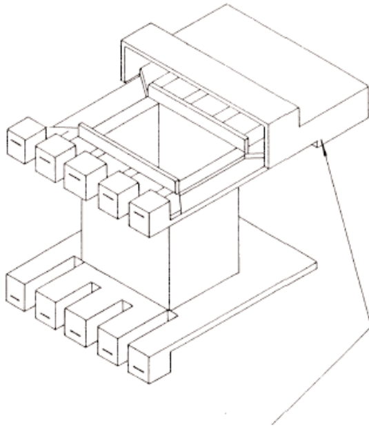
Insulator Fitted to One Bobbin Cheek
