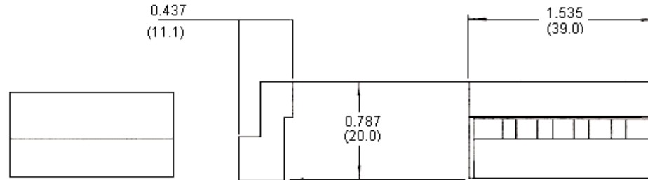
Pattern B for Use on Bobbin Sizes 35 and 147
