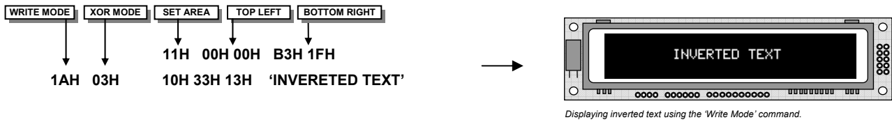
Displaying inverted text using the 'Write Mode' command.
