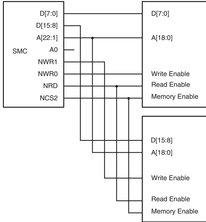
Figure 22-6. Memory Connection for 2 x 8-bit Data Path Devices
