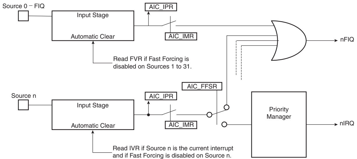
Figure 27-10. Fast Forcing
