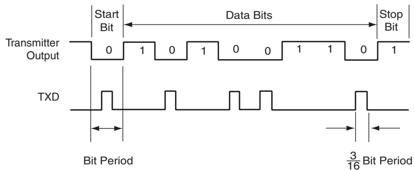
Figure 34-24. IrDA Modulation
