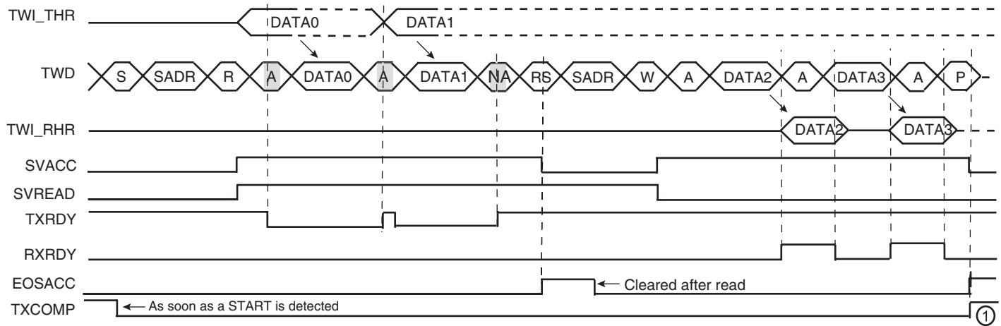
Figure 33-22. Repeated Start + Reversal from Read to Write Mode
