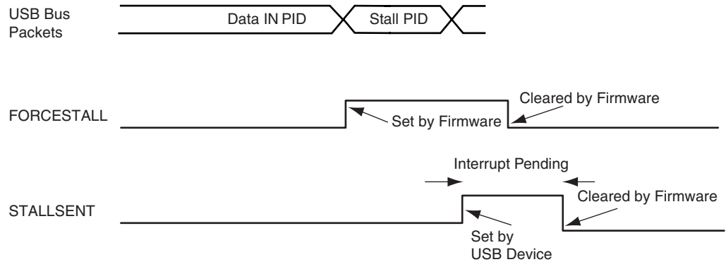
Figure 38-12. Stall Handshake (Data IN Transfer)
