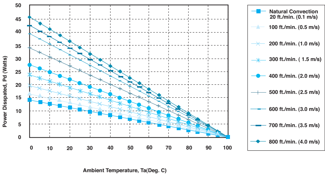
Forced Convection Power Derating without Heat Sink
