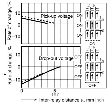
14.-(3) Influence of adjacent mounting
