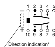
1-coil latching (Reset condition)
