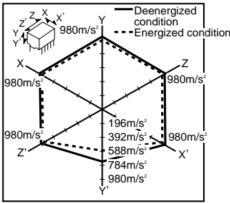
13.-(1) Malfunctional shock (single side stable) Tested sample: TF2-12V, 6 pcs
