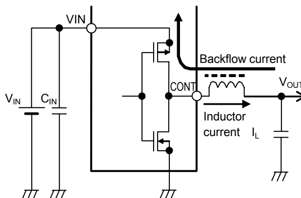
Figure 10 Backflow Current
