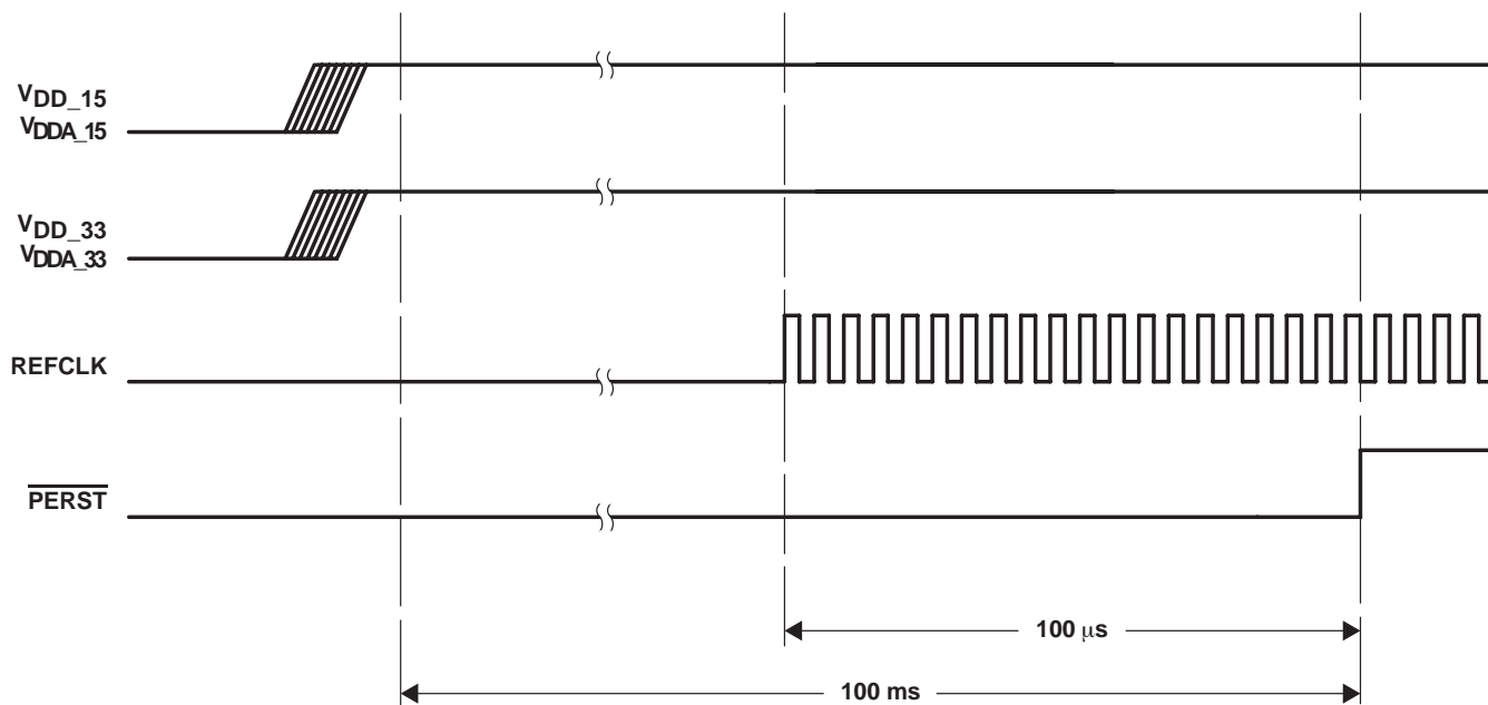
Figure 3–2. Power-Up Sequence
