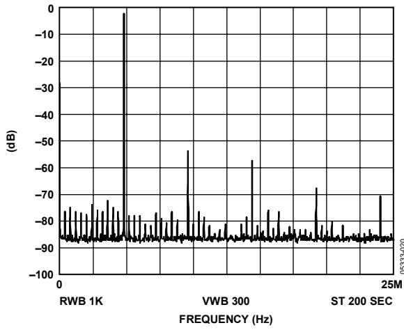
Figure 28. f_{MCLK} = 50 MHz; f_{OUT} = 4.8 MHz, Frequency Word = 189374C
