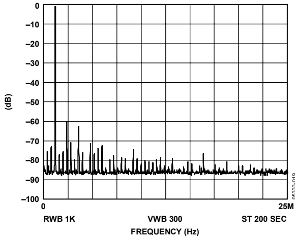
Figure 27. f_{MCLK} = 50 MHz; f_{OUT} = 1.2 MHz, Frequency Word = 0624DD3
