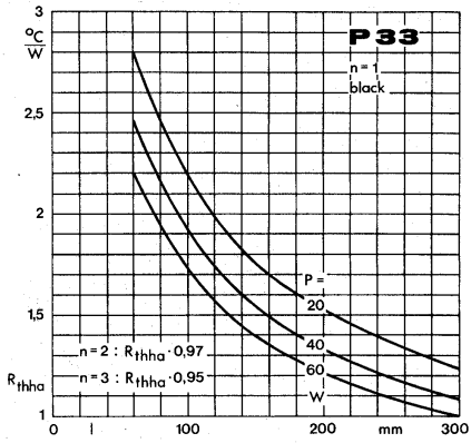
Fig. 2 Thermal resistance per component vs. length
