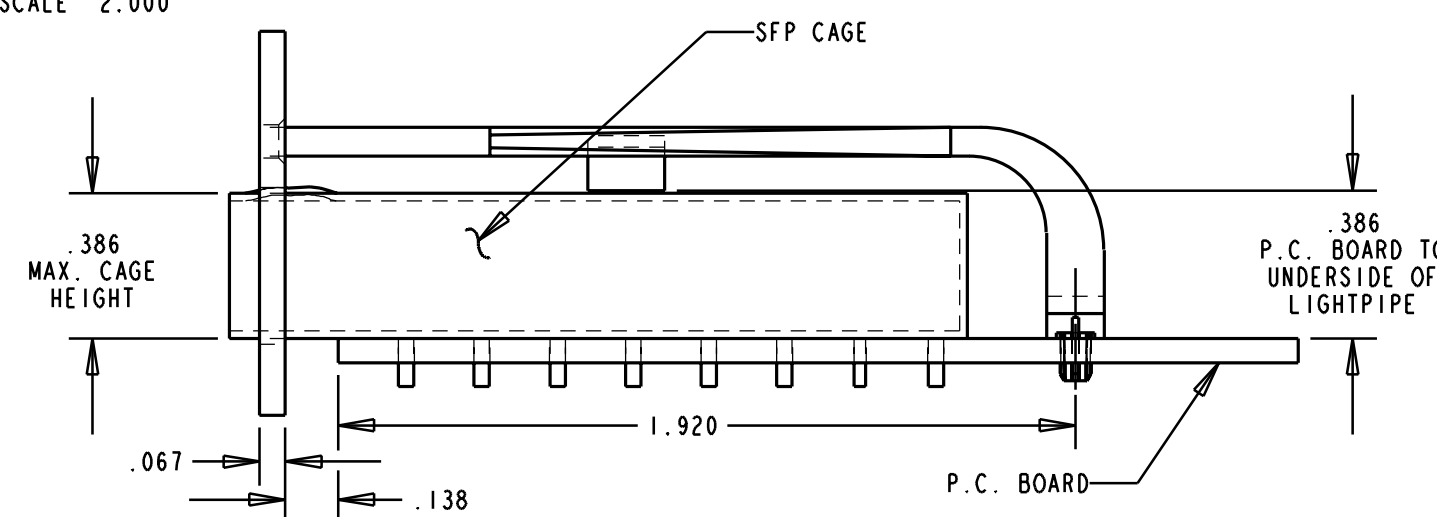
TYPICAL LIGHTPIPE APPLICATION USED WITH (SFP) CAGE ASSEMBLY SCALE 2.000
