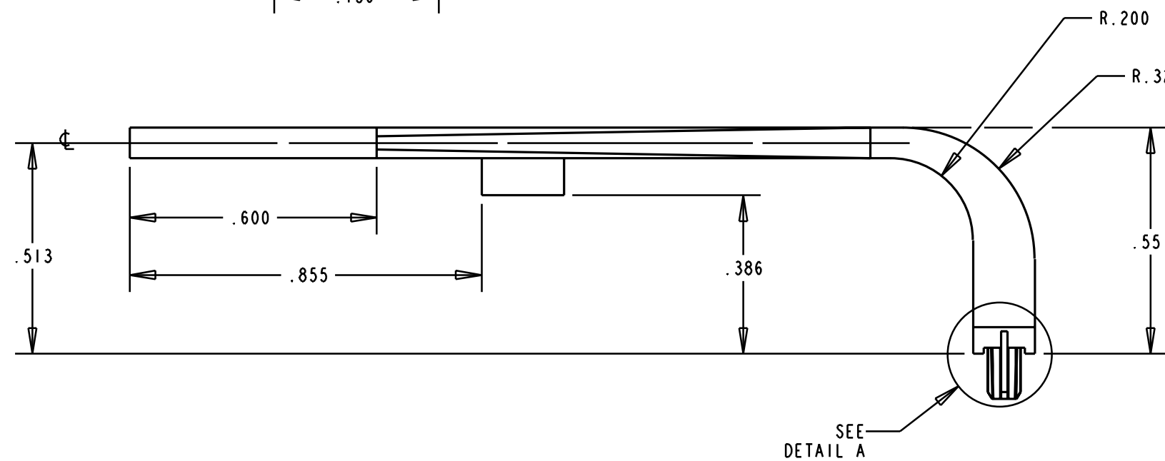
TYPICAL LIGHTPIPE APPLICATION USED WITH (SFP) CAGE ASSEMBLY SCALE 2.000
