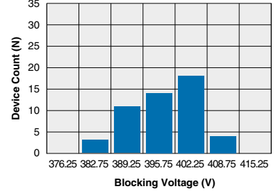
TS117L Typical Blocking Voltage Distribution (N=50 Ambient Temperature = 25°C)
