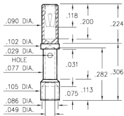
0348-0-33-XX-34-XX-10-0 #20A Crimp Barrel
