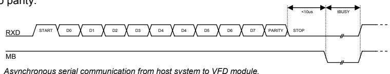
Asynchronous serial communication from host system to VFD module.
