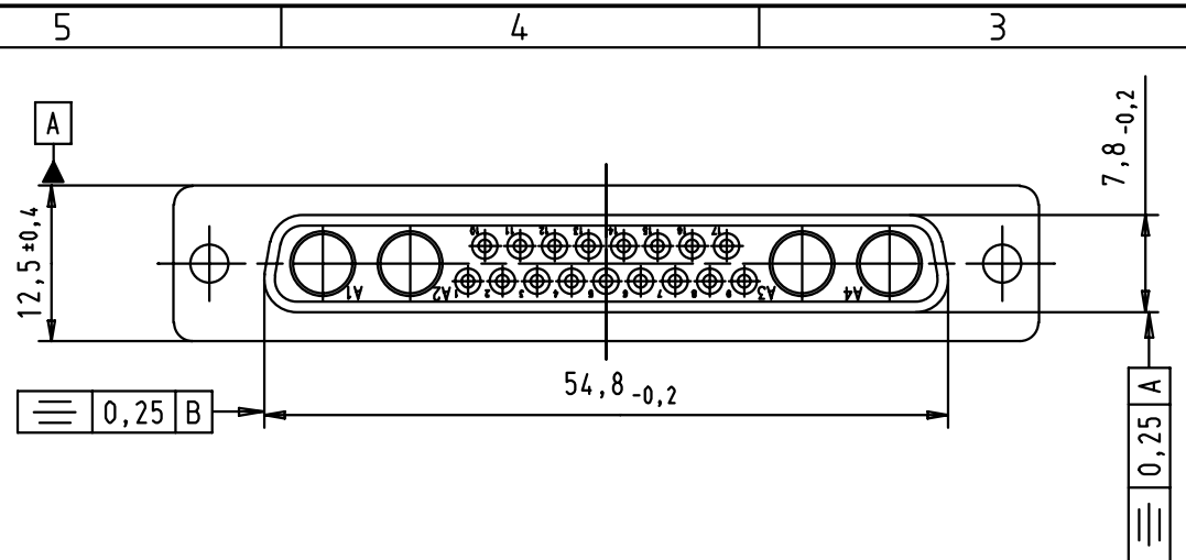
Solder bucket termination for AWG 20 (0.5 mm 2 )
