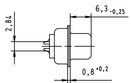
Solder bucket termination for AWG 20 (0.5 mm 2 )
