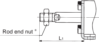
Front flange/CQ2F
