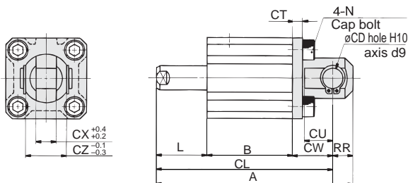
Double clevis/CQ2D
