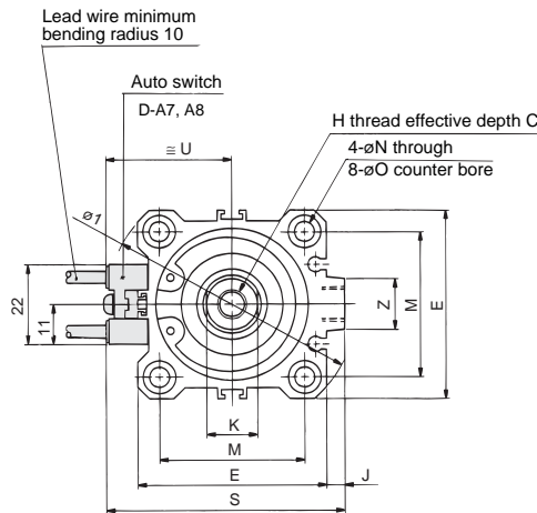
Standard (Through-hole)/CQ2B, CDQ2B
