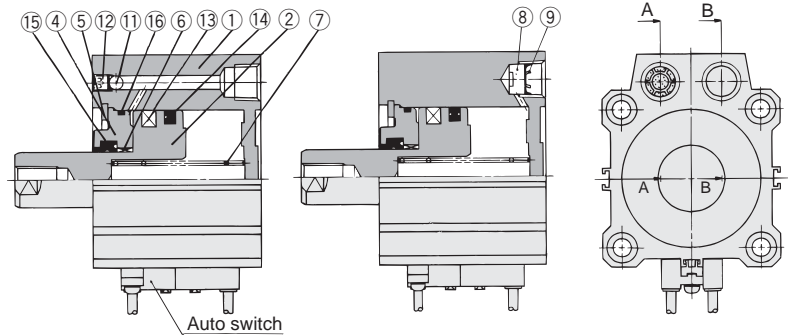
A-A section (Rod side port) B-B section (Head side port) A-A section (Rod side port) B-B section (Head side port)
