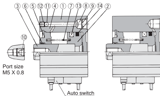
A-A section (Rod side port) B-B section (Head side port) A-A section (Rod side port) B-B section (Head side port)
