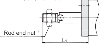
Rear flange/CQ2G
