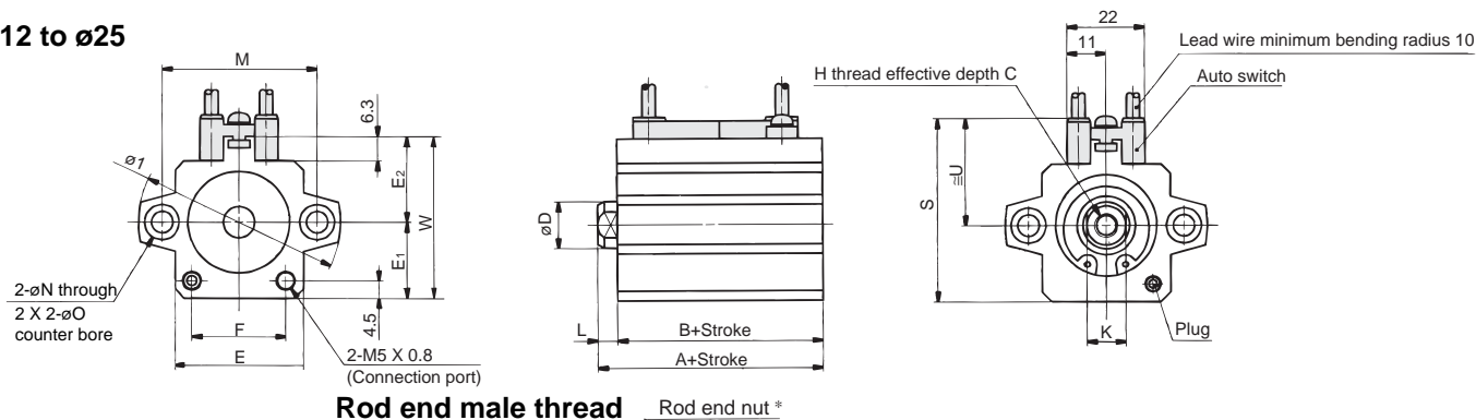
Rod end male thread (mm)
