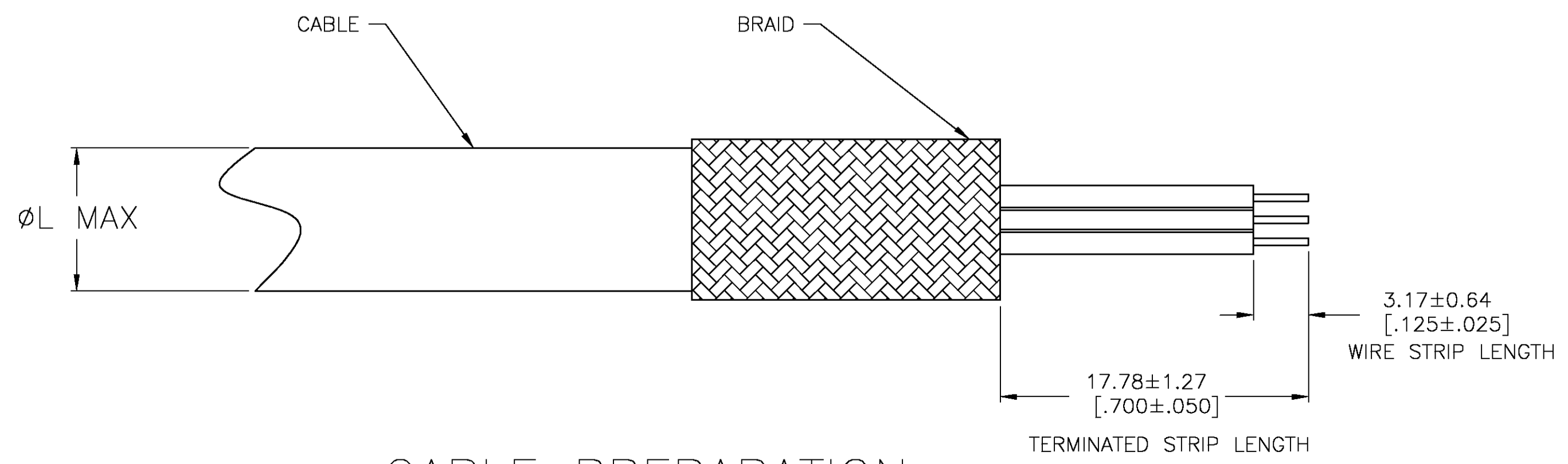
CABLE PREPARATION
