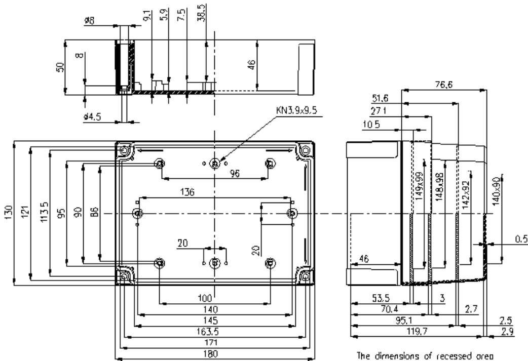
The dimensions of recessed area on top of cover have been given above ( e.g. 149x99 ). The area have radius 2.0 mm in the corners.
