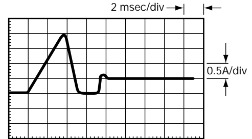
Fig. 6a. Switch-on pulse and steady-state current, example #6.
