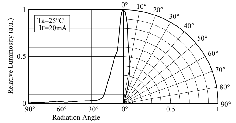
■ Directivity (NSPG300A)
