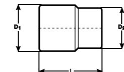
Hexagon sockets, 1/4"
