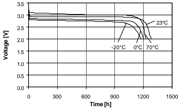
Temperature performance Load 6.81kW
