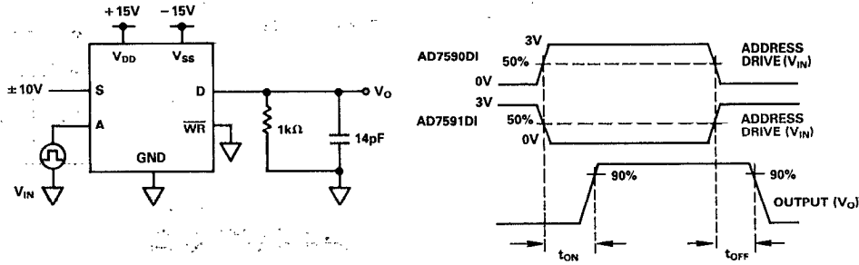
TEST CIRCUIT 6 SWITCHING TIME OF AD7592DI, t_{TRANSITION}
