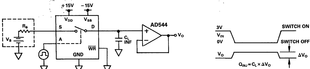
TEST CIRCUIT 7 CHARGE INJECTION
