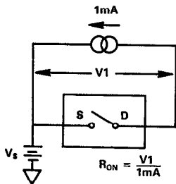
TEST CIRCUIT 3
