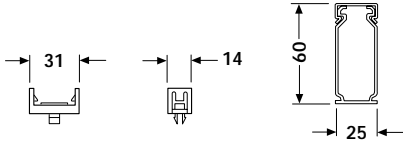
Duct 25x60 mm
