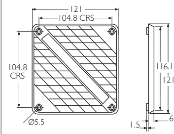
FG120T Moulded plastic guard. 4xxx and 9xxx series fans
