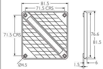
FG80T Moulded plastic guard. 8xxx series fans
