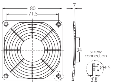
LZ32-2 Black, fibre-glass reinforced plastic. 8xxx series fans
