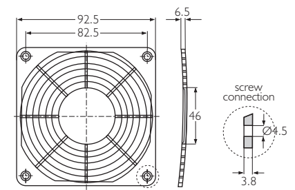
LZ23-2 Black, fibre-glass reinforced plastic. 3xxx series fans
