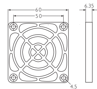
LZ28P Plastic UL Listed 94-VO. 6xx series fans
