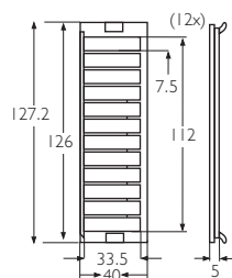
LZ34 Special plastic guard for radial blowers. RG series fans
