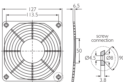
LZ33-1 Black, fibre-glass reinforced plastic. 5xxx series fans
