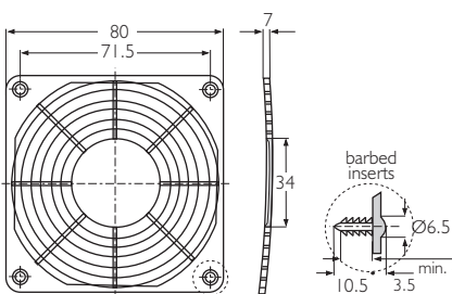
LZ32-3 Black, fibre-glass reinforced plastic. 8xxx series fans
