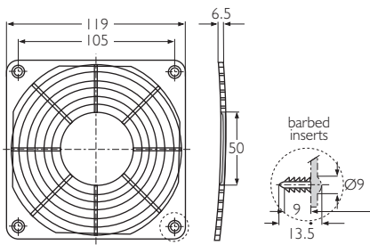
LZ30-6 Black, fibre-glass reinforced plastic. 4xxx and 9xxx series fans
