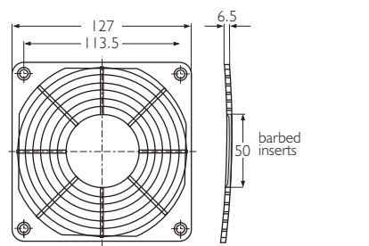
LZ33-2 Black, fibre-glass reinforced plastic. 5xxx series fans
