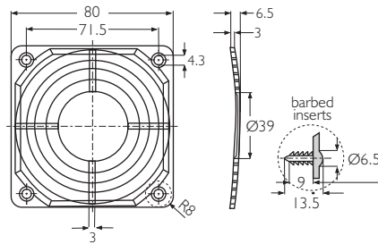
LZ32P Black, fibre-glass reinforced plastic. 8xxx series fans
