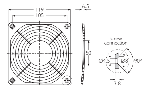
LZ30-5 Black, fibre-glass reinforced plastic. 4xxx and 9xxx series fans
