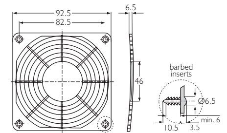
LZ23-3 Black, fibre-glass reinforced plastic. 3xxx series fans
