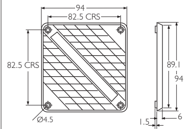
FG92T Moulded plastic guard. 3xxx series fans
