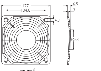
LZ30P Black, fibre-glass reinforced plastic. 4xxx and 9xxx series fans
