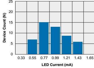
IAB110P - FormB Typical I F for Switch Operation (N=50 Ambient Temperature = 25°C) (Load Current = 100mADC)
