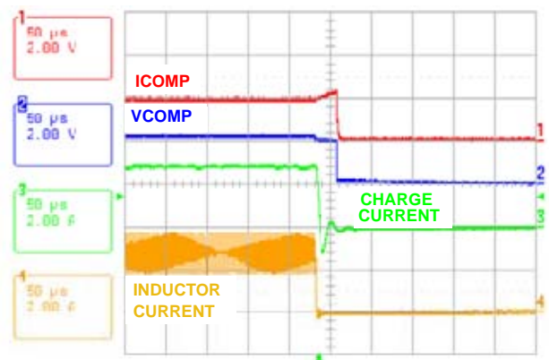
FIGURE 8. CHARGE DISABLE
