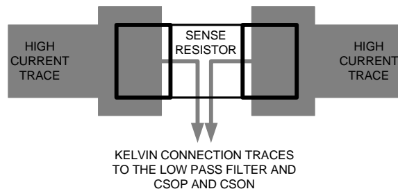
FIGURE 26. CURRENT SENSE RESISTOR LAYOUT
