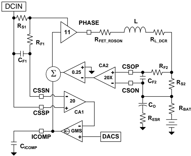
FIGURE 22. ADAPTER CURRENT LIMIT CONTROL LOOP
