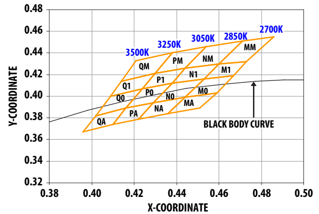
Figure 26. Color bin structure for Warm White
