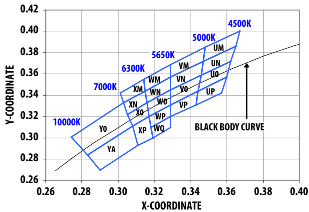
Figure 25. Color bin Structure for Cool White
