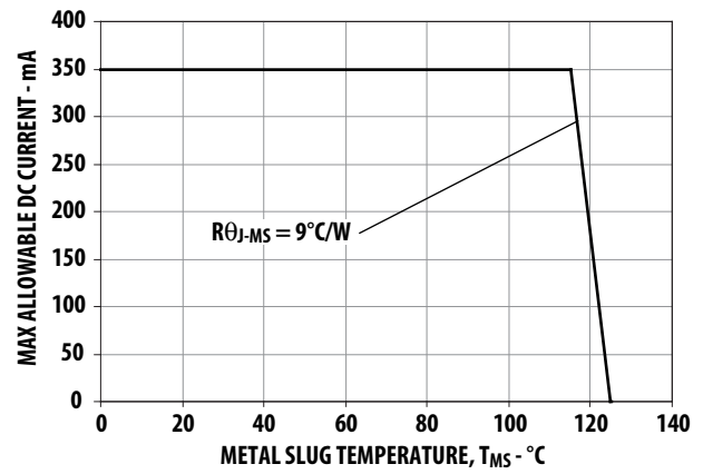
Figure 10. Maximum Forward Current vs. Ambient Temperature. Derated based on T JMAX = 125°C, R θJ-MS = 9°C/W
