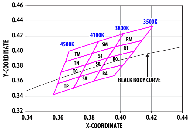
Figure 27. Color bin structure for Neutral White
