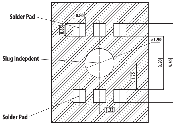
Figure 23. Recommended soldering land pattern
