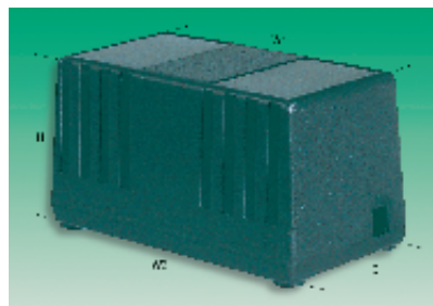
H = 62, W 1 = 112, W 2 = 117, D = 63
