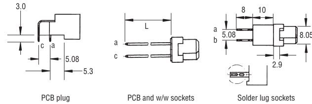
Pin spacing = 5.08 PCB hole dia. = 1.0
