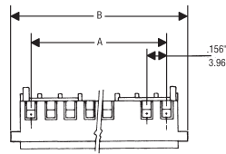
A = Number of ways — 1 3.96 (0.156") B = A+4.42
