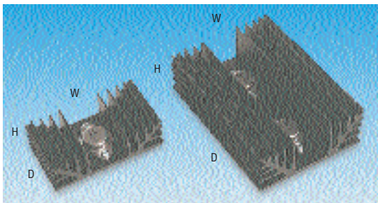
253-698 H = 25, W = 88, D = 50
