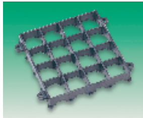
Support bracket L = 62.5, W = 62.5, D = 10.5 Fixing centres = 45.72 68.0
