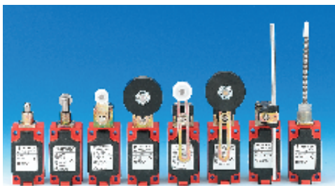
Body H = 73.5 (excluding head), W = 40, D = 40 Fixing centres = 60 30mm
