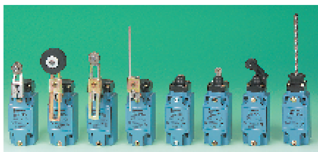
Roller lever Large roller lever Adjustable roller lever Adjustable rod lever Pin plunger Roller plunger Roller arm Coil spring
