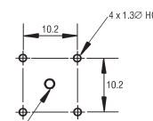
Stepped PCB drilling patterns
