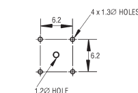
Straight PCB drilling patterns
