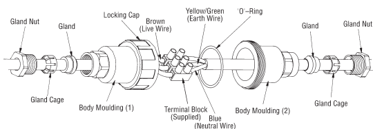
L = 105, Dia = 38
