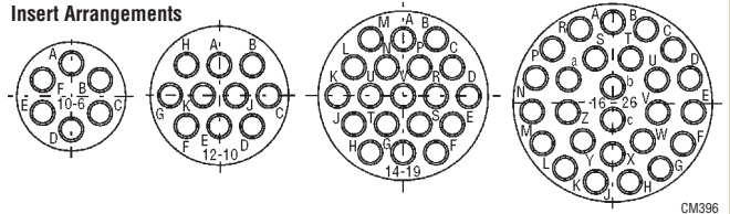
890-492 Socket Housing
